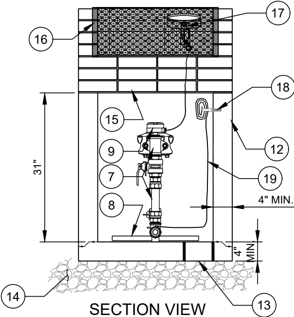
ALTERNATE IN CONCRETE SIDEWALK
