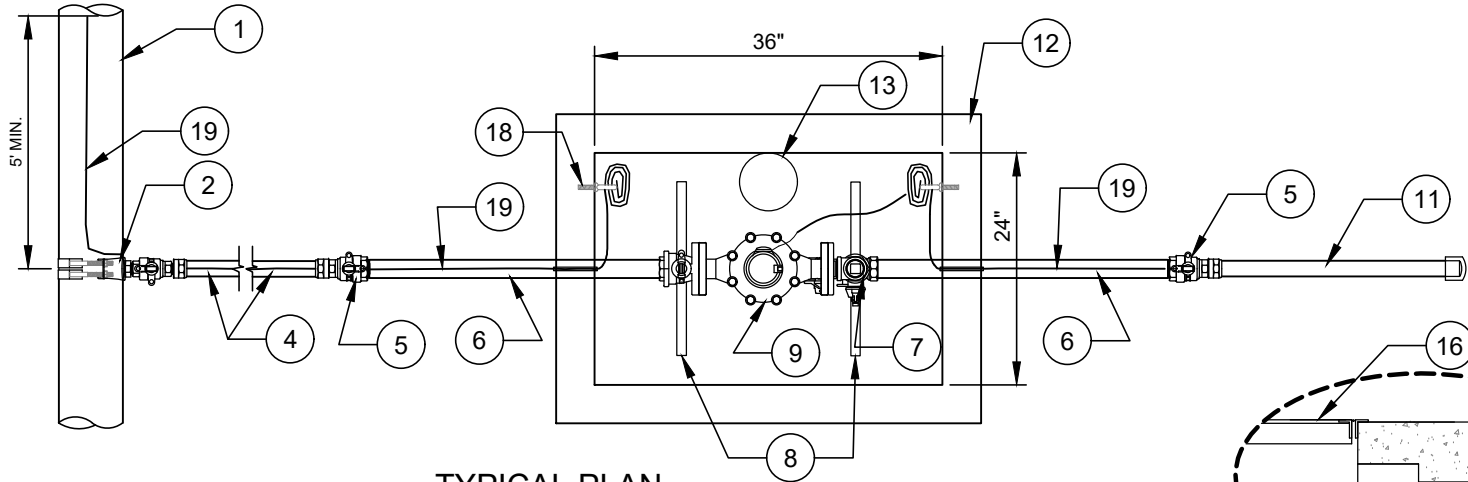
TYPICAL PLAN
