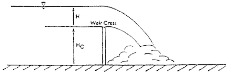
Figure 6-3 Sharp-Crested Weir
