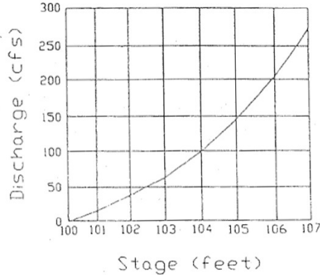
Figure 6-2 Example Stage-Discharge Curve
