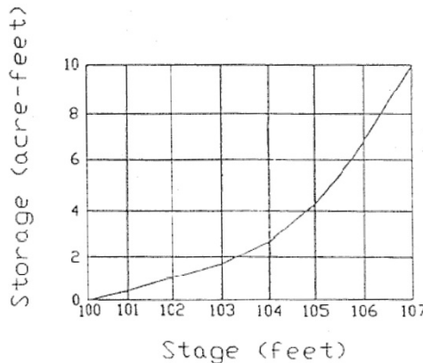
Figure 6-1 Example Stage-Storage Curve
