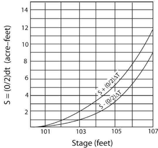
Figure 6A-1 Storage Characteristics Curve
