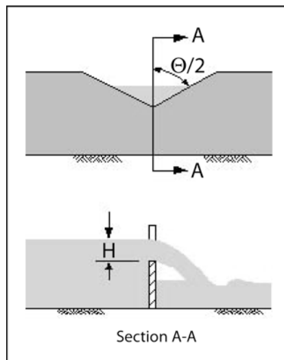
Figure 6-5 V-Notch Weir
