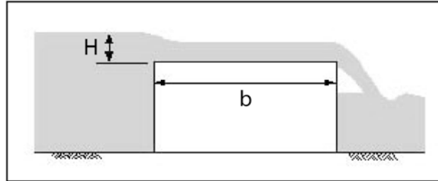
Figure 6-4 Broad-Crested Weir
