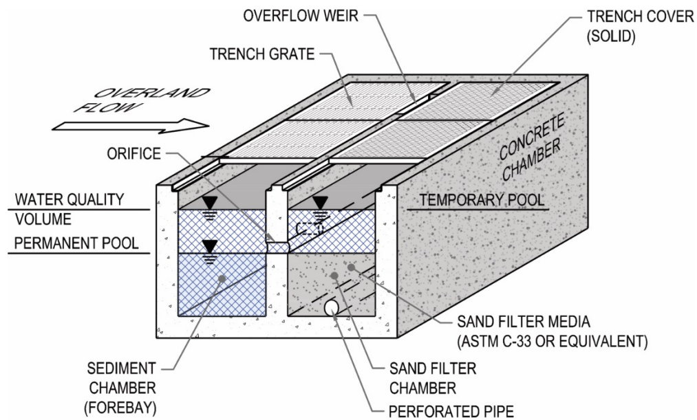
Figure 2: Closed Bottom Sand Filter Example: Cross-Section
