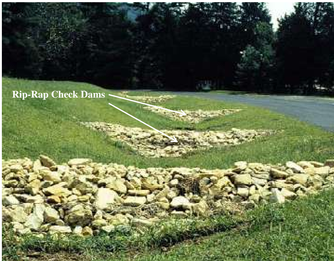
Figure 6.2 Grass Swale with Check Dams
