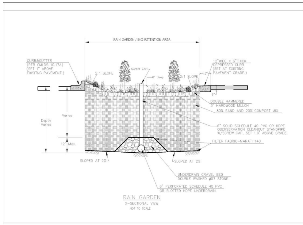
Figure 2: Bioretention Cell Design Profile
