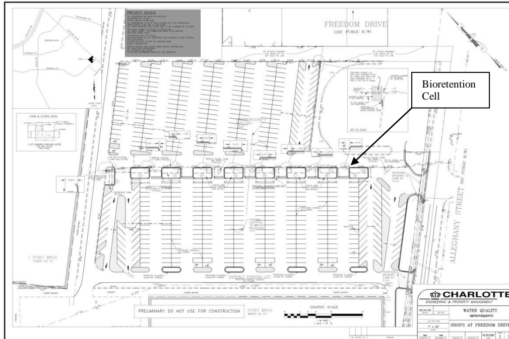
Figure 1: Shops on Freedom Drive Plan View Layout
