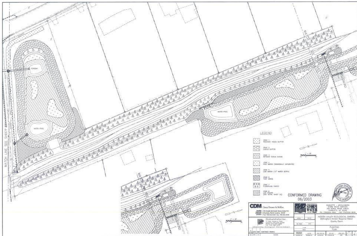
Figure 2: Wellington Wetland Planting Plan
