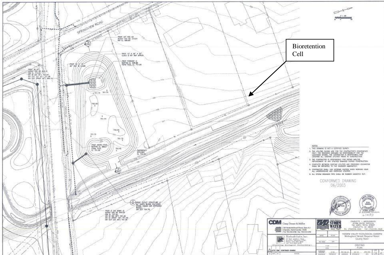
Figure 1: Wellingford Wetland Plan View Layout
