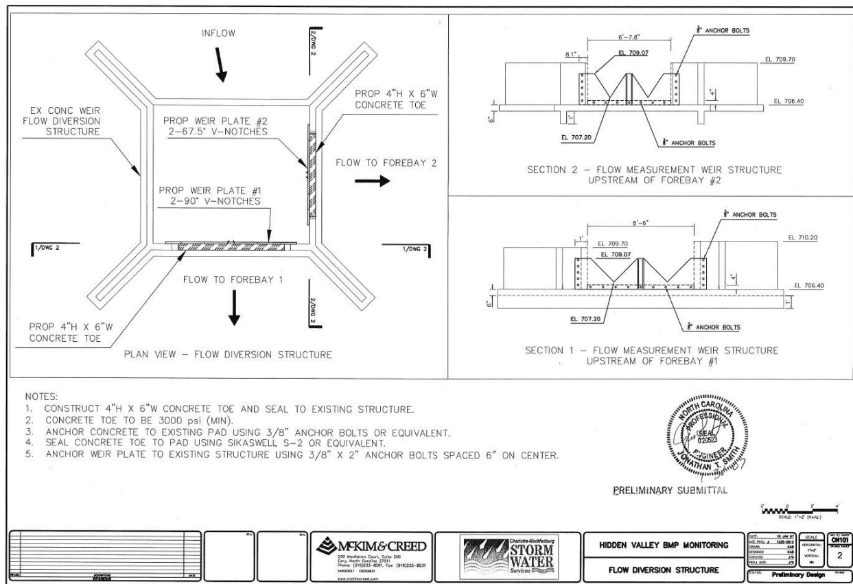
Figure 2: Inlet weir flow splitter design
