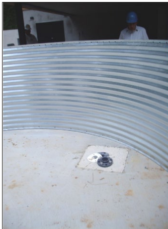
Figure 3. Metal cistern under construction (left), underground concrete vault wrapped in an impermeable liner (center) and a series of plastic cisterns (right) (UNC-CH left and NCSU BAE center and right)
