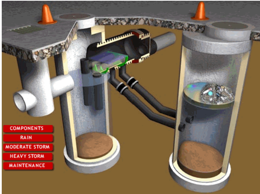
Figure 3: BaySeparator Unit
