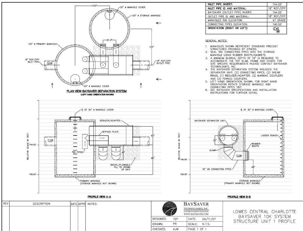
Figure 2: BaySeparator Details
