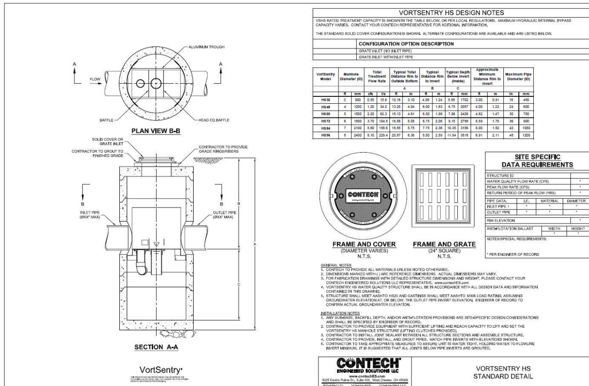
Figure 2: Vort Sentry Detail
