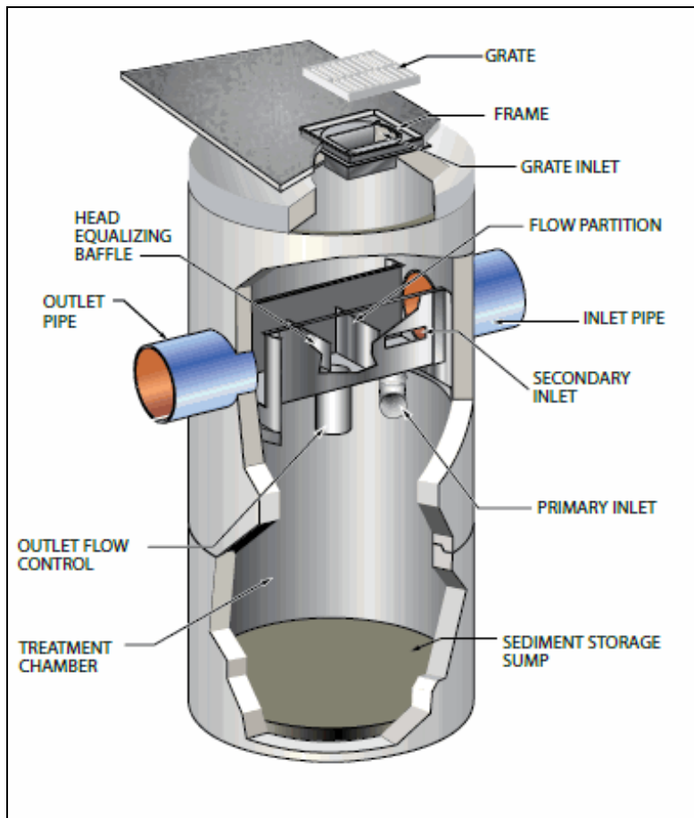
Figure 3: Vort Sentry Unit
