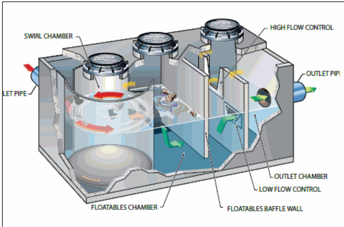
Figure 3: Vortechinics Unit
