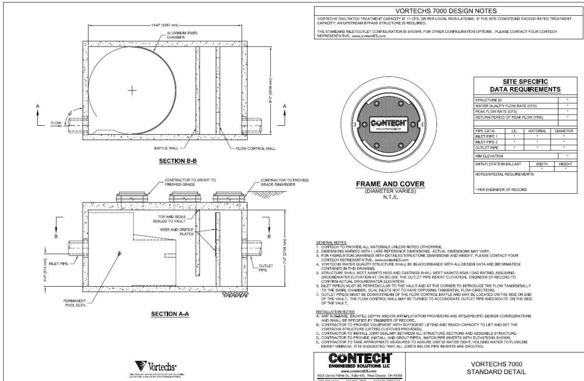
Figure 2: Vortechics Detail
