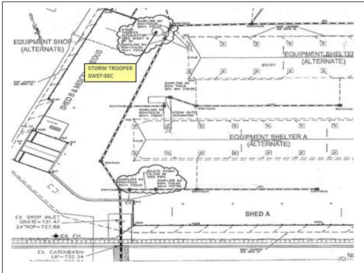
Figure 1: CDOT North Pointe Storm Trooper - Plan View Layout
