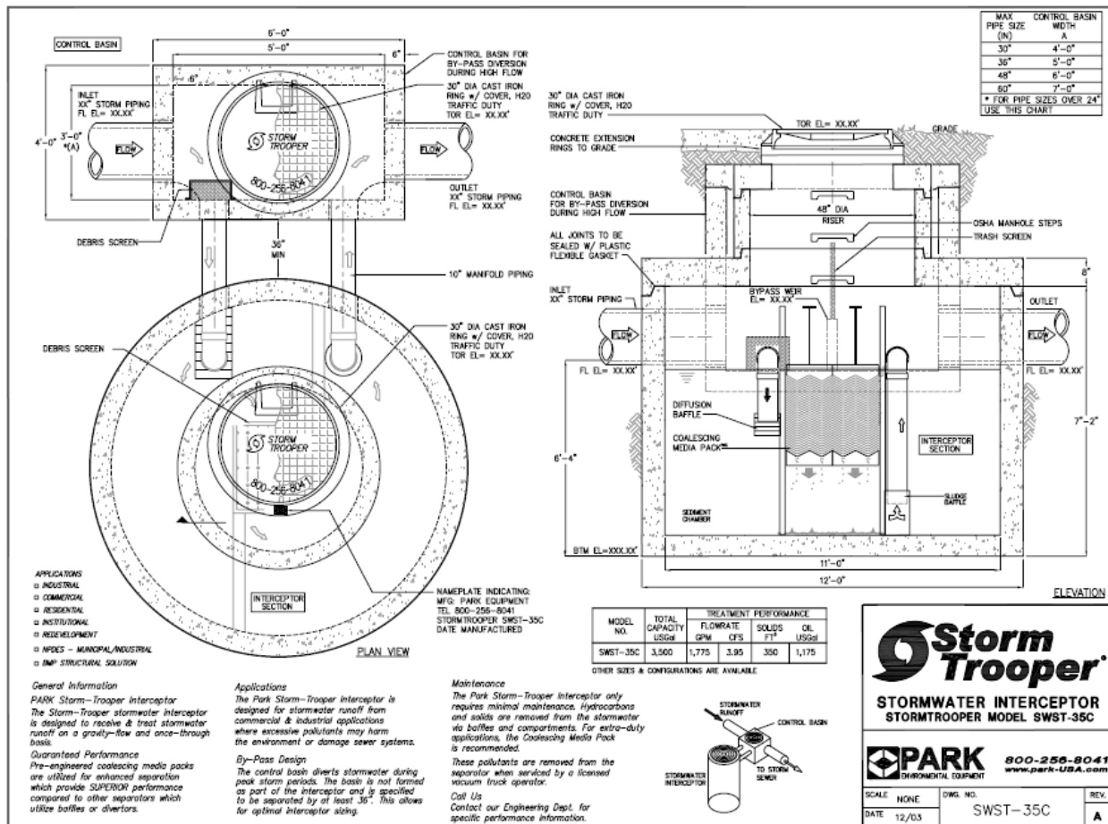
Figure 2: Storm Trooper SWST-35C 1
