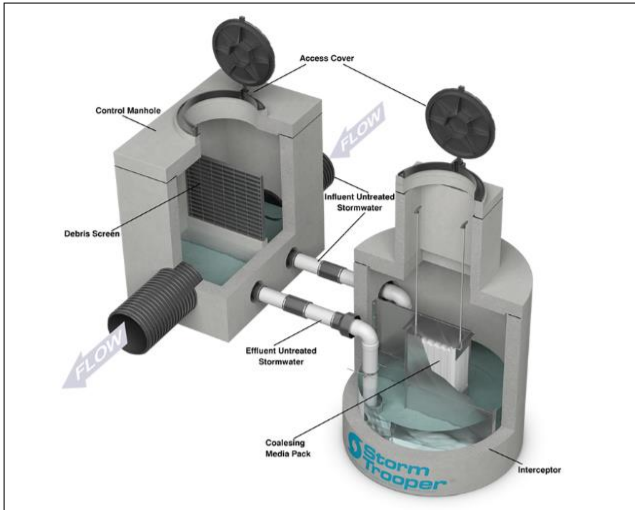
Figure 3: Storm Trooper Unit 1
