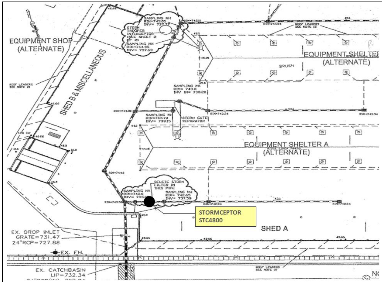
Figure 1: CDOT North Pointe StormCeptor - Plan View Layout
