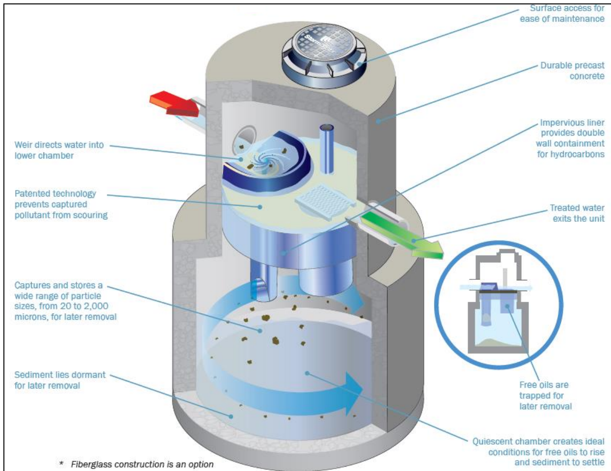
Figure 3: StormCeptor Unit 1 .
