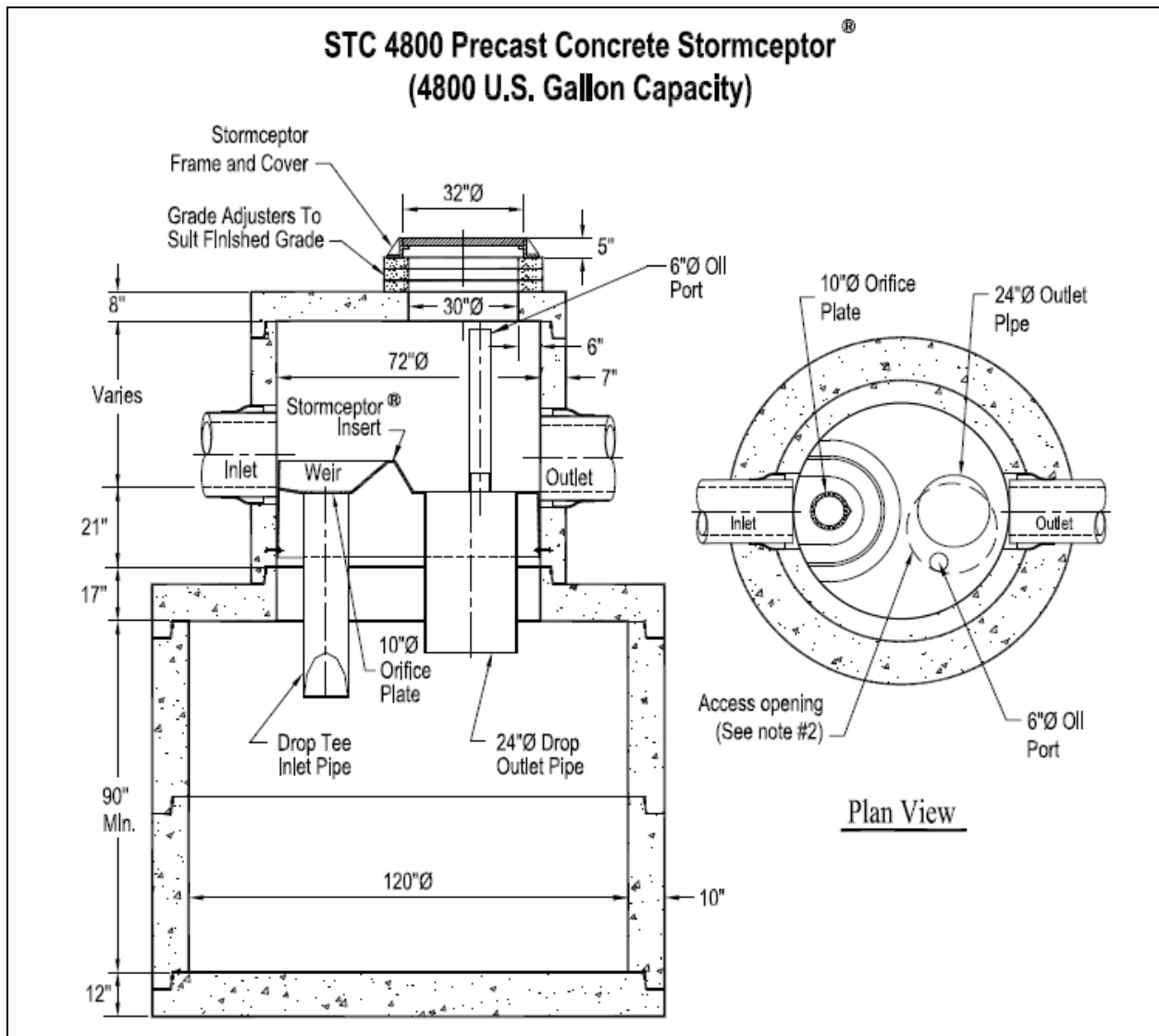
Figure 2: StormCeptor STC4800 Detail 1 .
