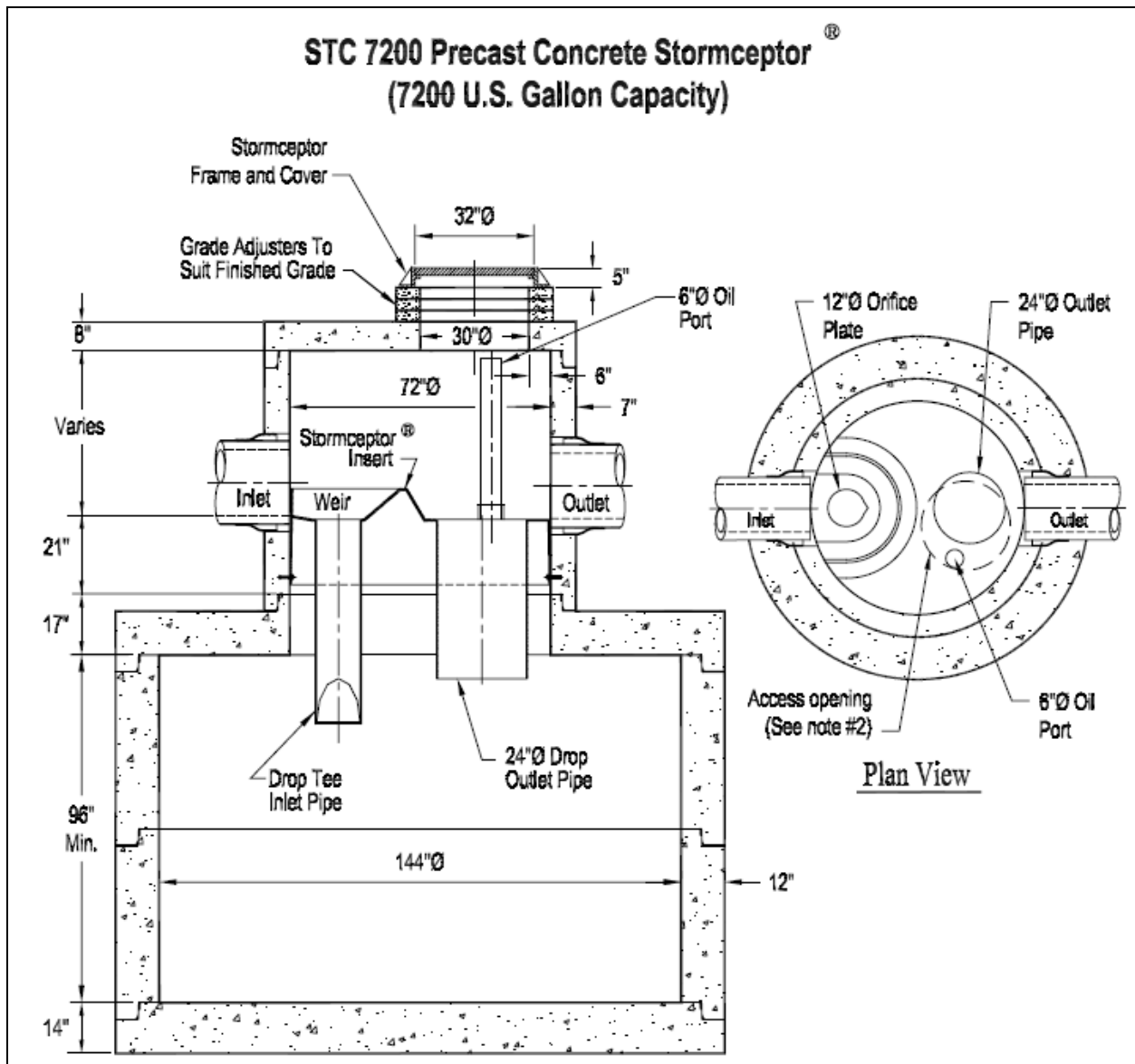
Figure 2: StormCeptor STC7200 Detail 1 .
