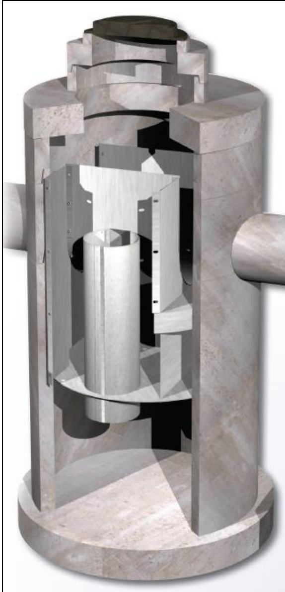
Figure 3: FloGard DVS Unit 1
