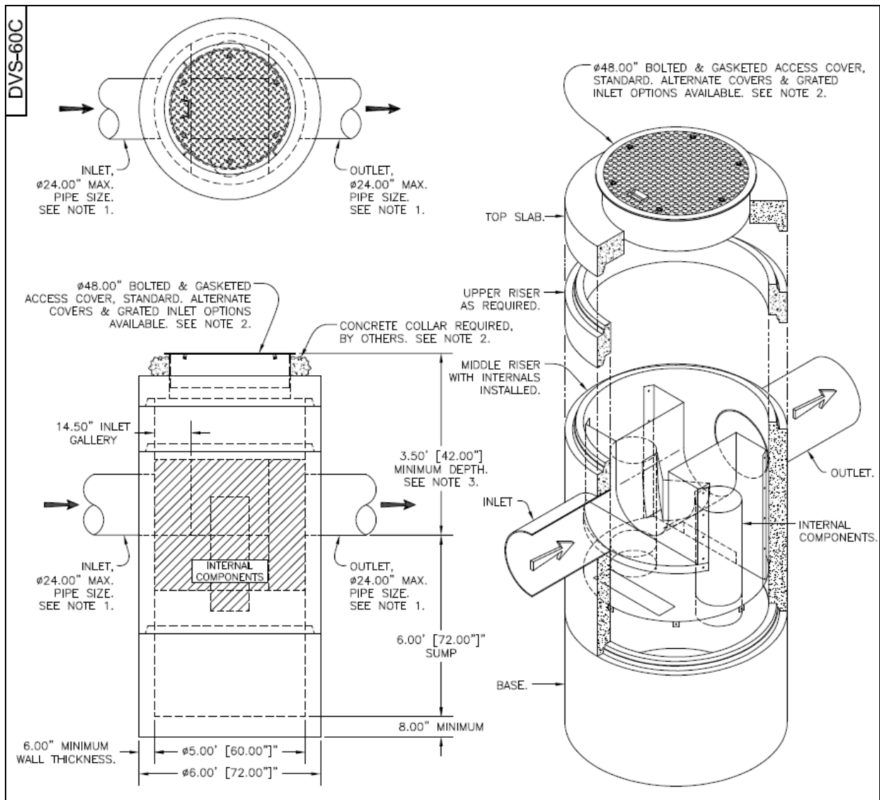
Figure 2: FloGard DVS-60 Detail 1 .
