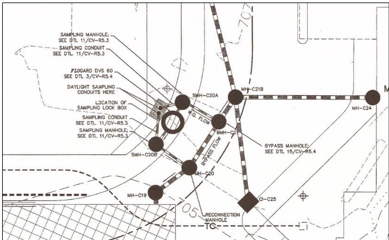
Figure 1: Ashley Park FloGard DVS - Plan View Layout
