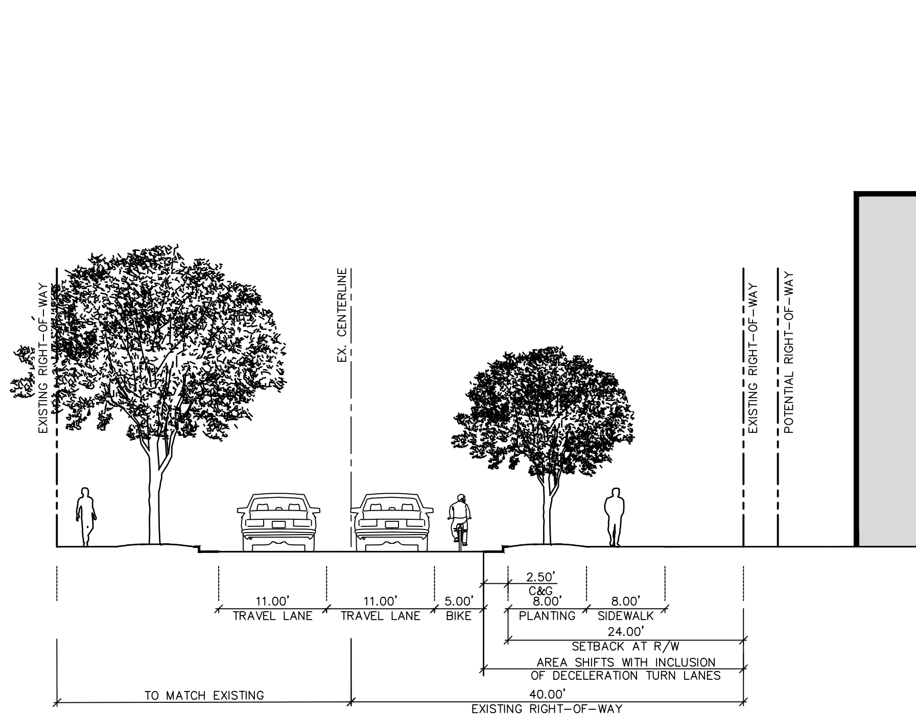
N. TRYON STREET CROSS SECTION
