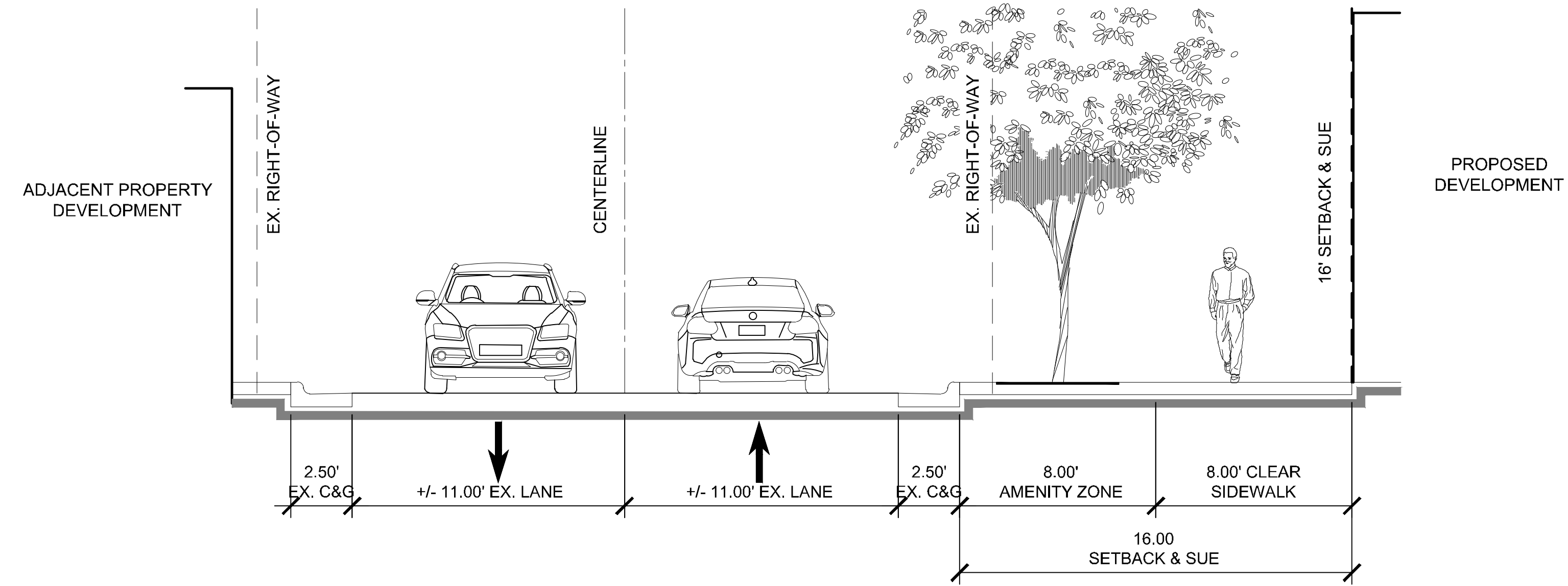
01 HEATH CT. PROPOSED CROSS SECTION SITE SECTION
