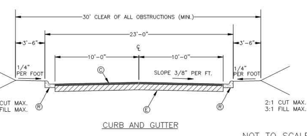
PRIVATE STREET TYPICAL SECTIONS NOT TO SCALE
