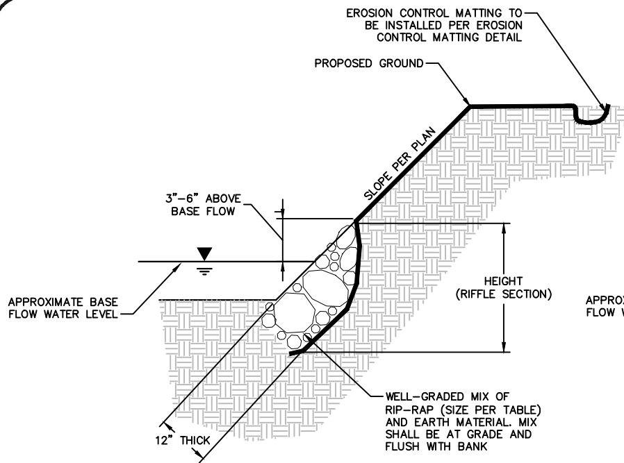
RIFFLE SECTION
