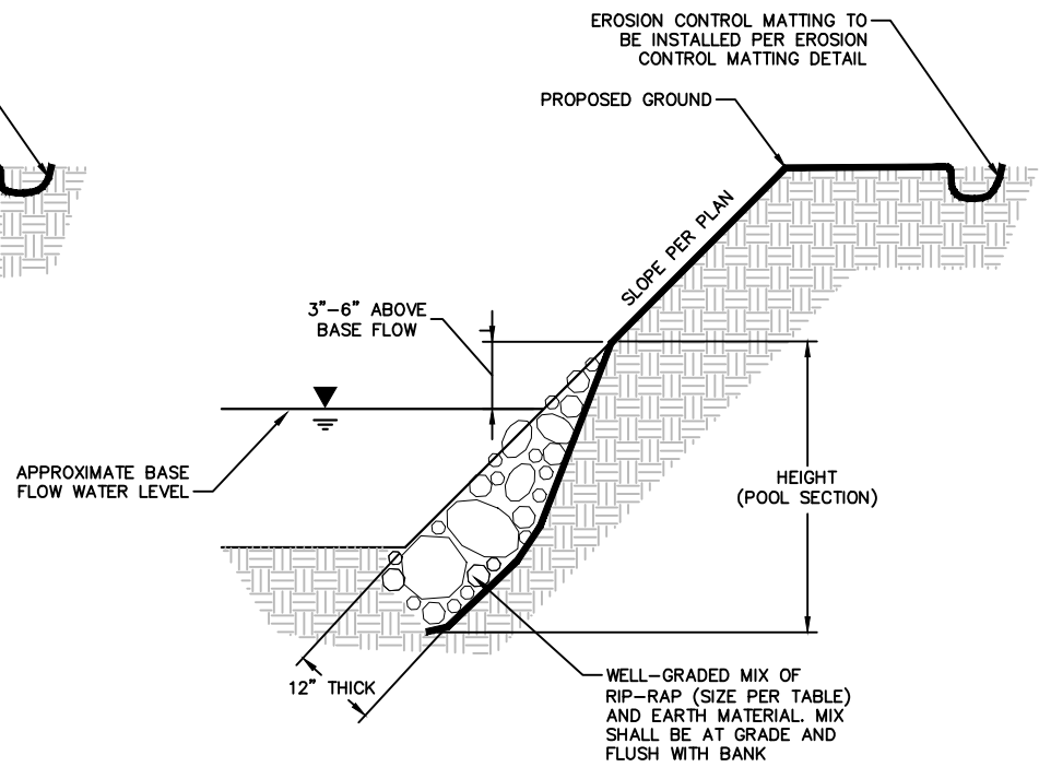
POOL SECTION
