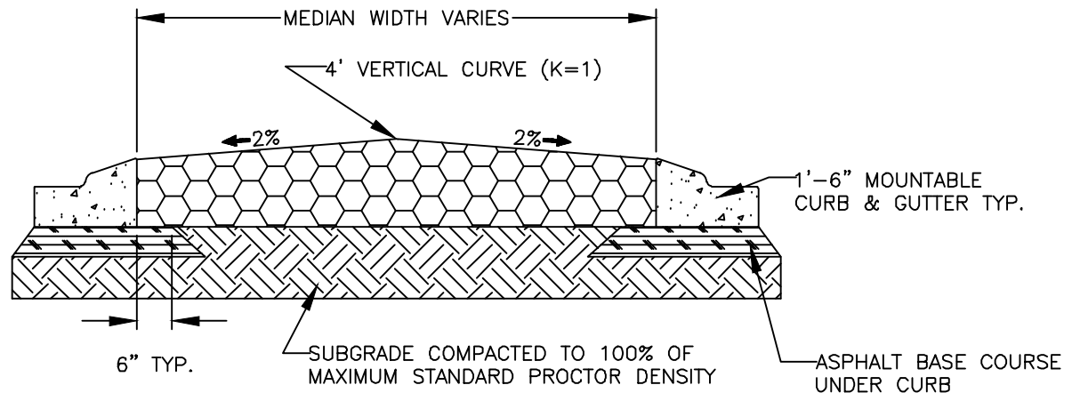
CROSS-SECTION X-X
