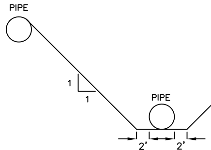
PROFILE VIEW
